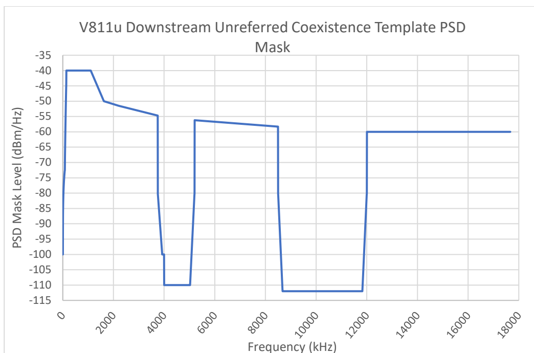
FIGURE 5 V811u Downstream Unreferred Coexistence Template PSD Mask
