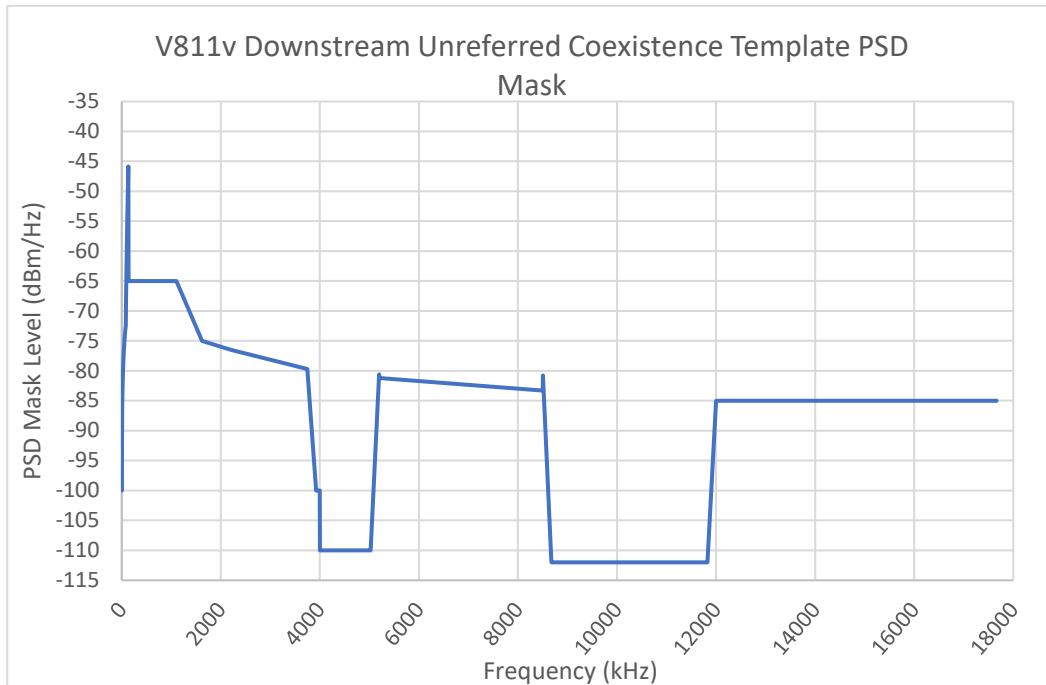
FIGURE 11 V811v Downstream Unreferred Coexistence Template PSD Mask
