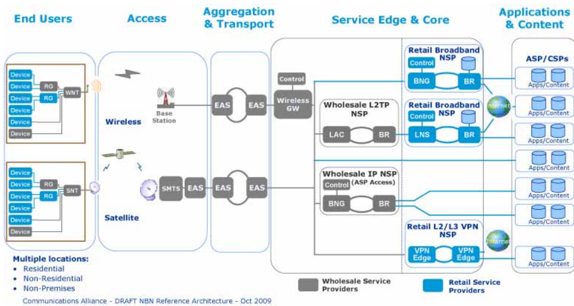
Figure 6 Network Reference Architecture – Wireless/Satellite Layer 2 Ethernet
