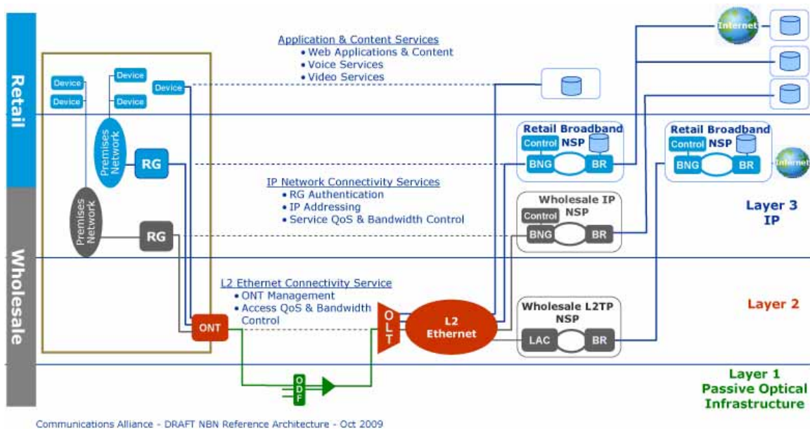
Figure 5 CPE Service Relationships
