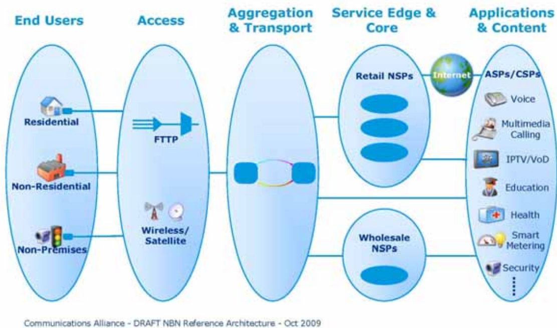
Figure 1 Broadband Network Architecture Vision
